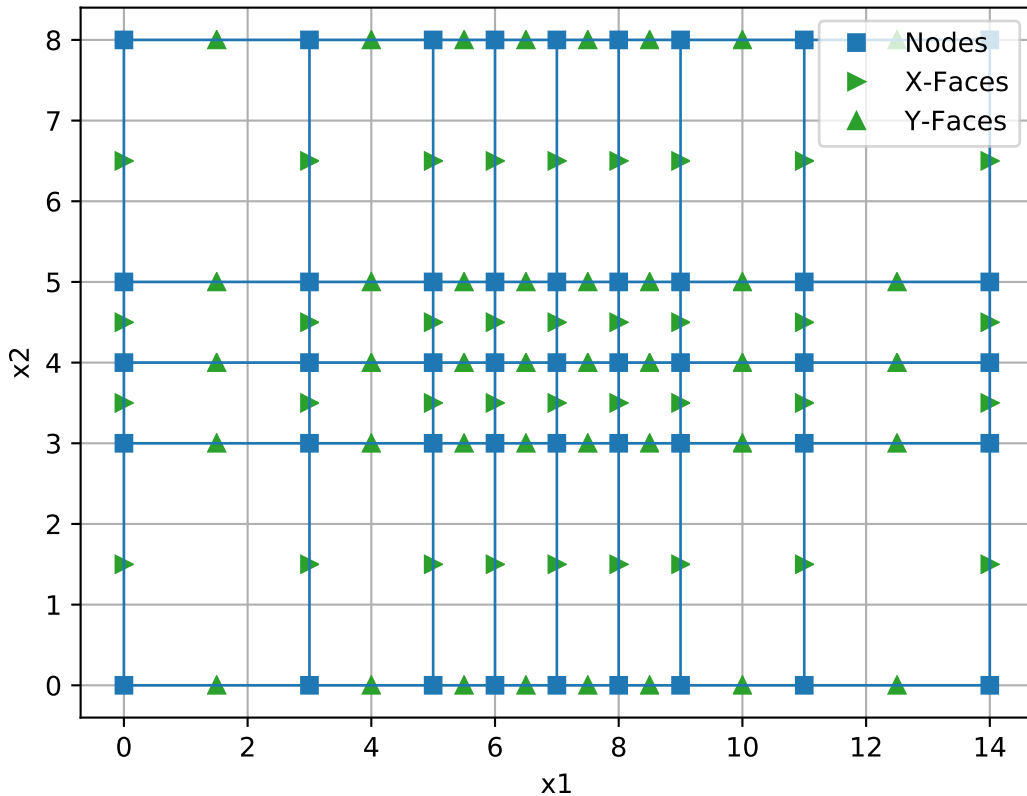
Cell faces in the x- and y-directions.
